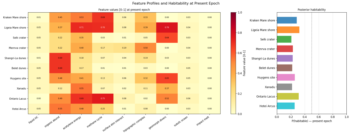
Figure 3.6: Feature profiles and posterior habitability for ten key sites. Left: heatmap of normalised feature values. Right: posterior mean P(H | f) ; dashed line = prior mean. Selk’s exceptional geodiversity ( f_7=0.629 ) is clearly visible despite its below-average aggregate score.
